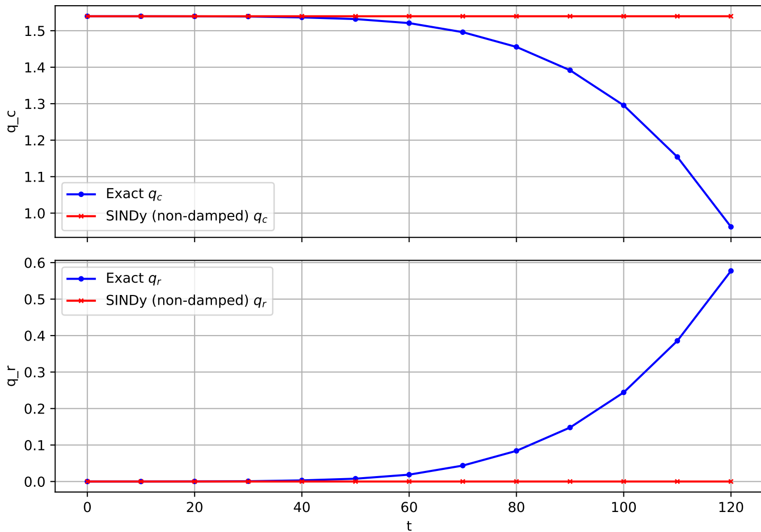
Trajectory 1592 (non-damped)
