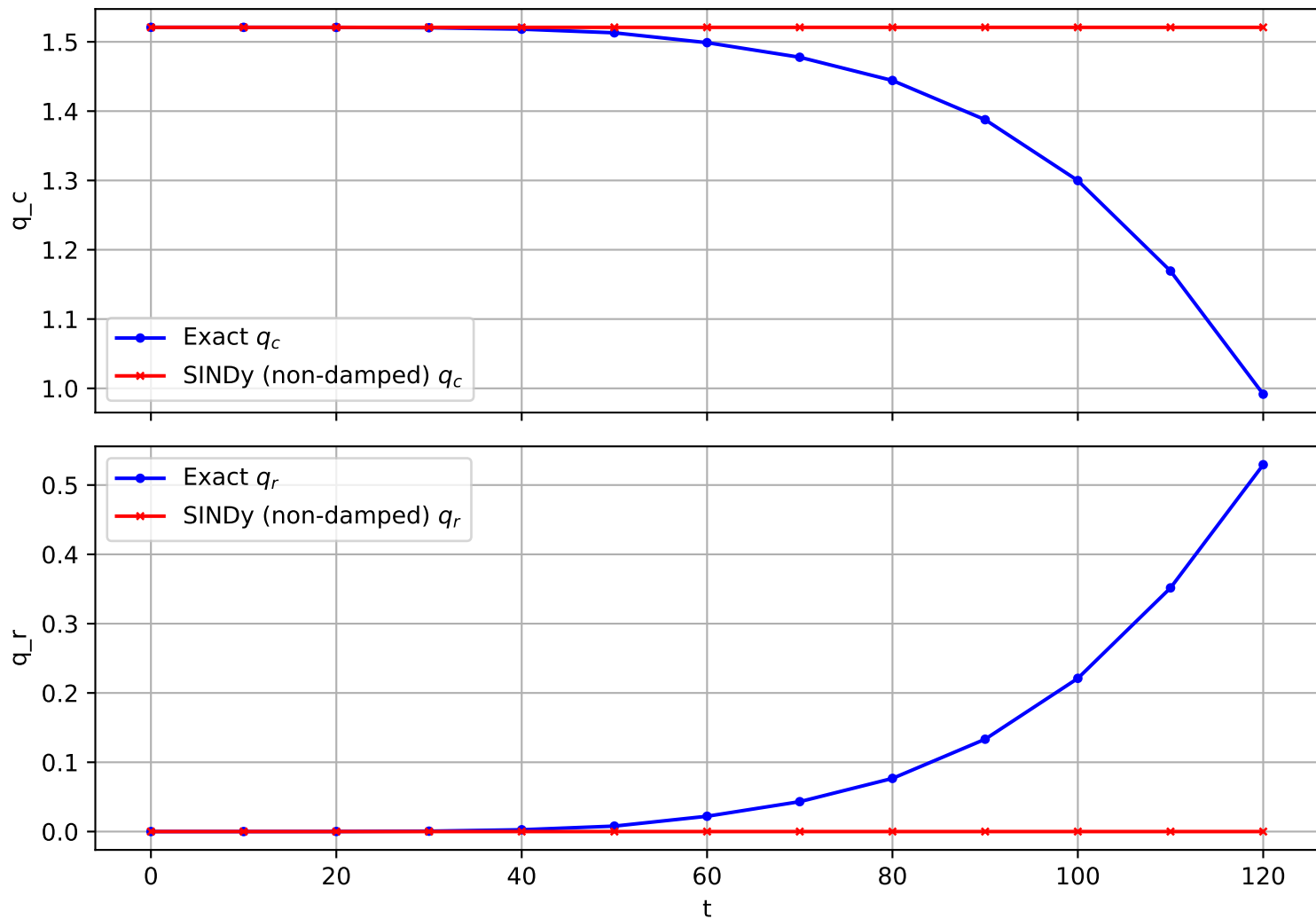
Trajectory 1593 (non-damped)
