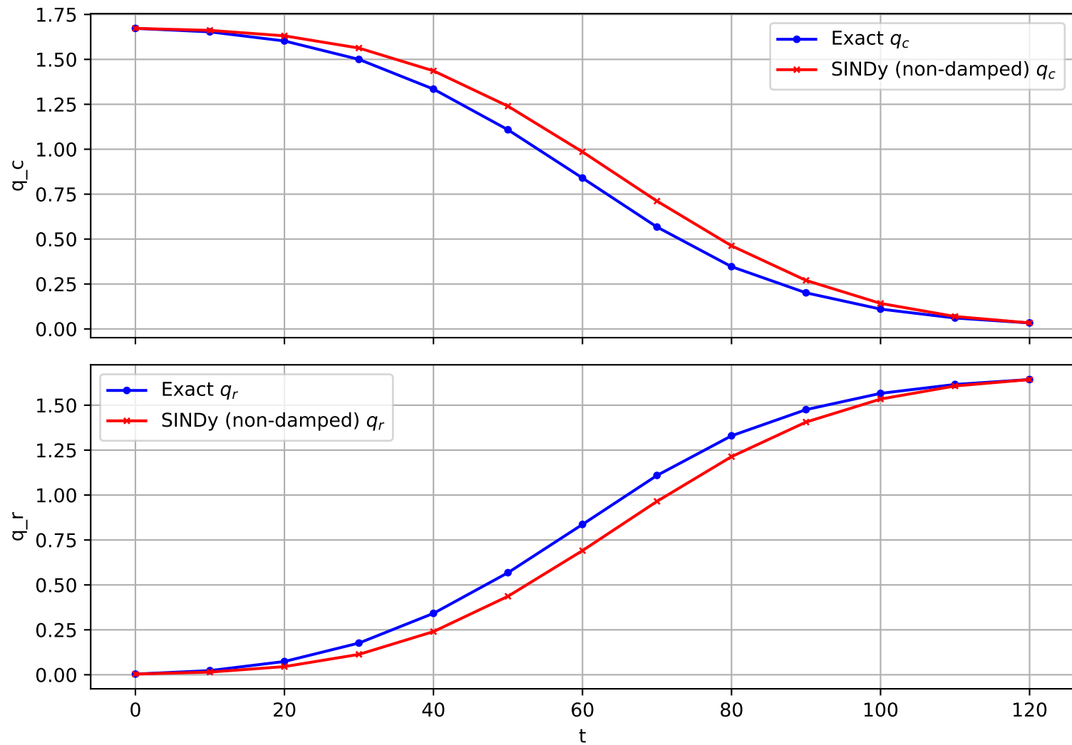
Trajectory 1601 (non-damped)
