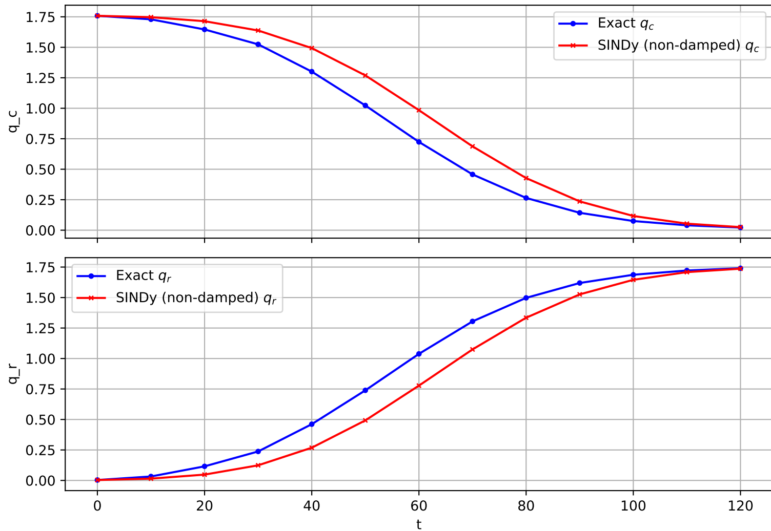
Trajectory 1602 (non-damped)
