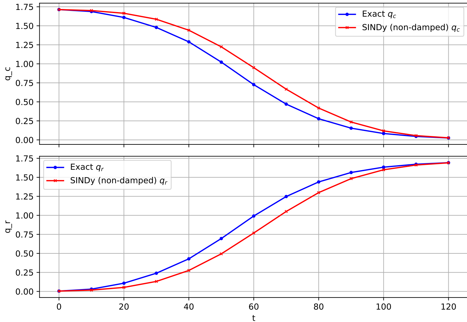
Trajectory 1604 (non-damped)
