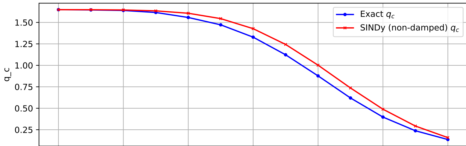
Trajectory 1613 (non-damped)
