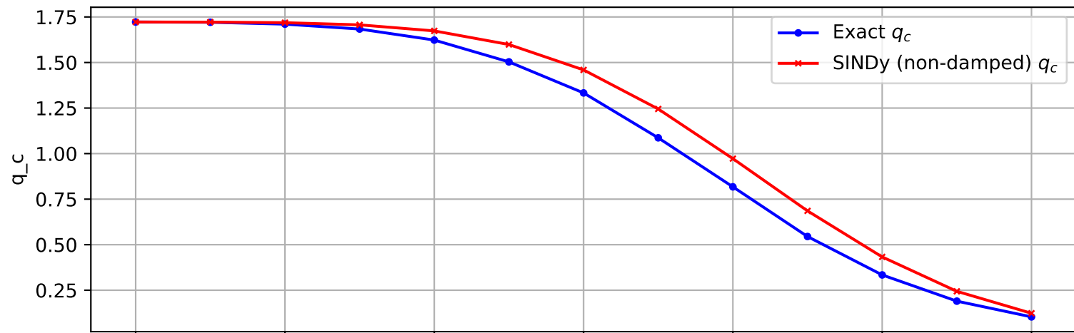
Trajectory 1614 (non-damped)
