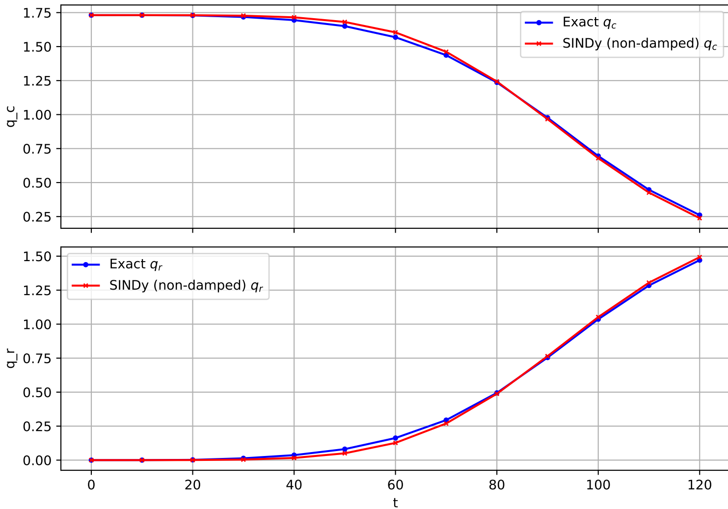
Trajectory 1617 (non-damped)
