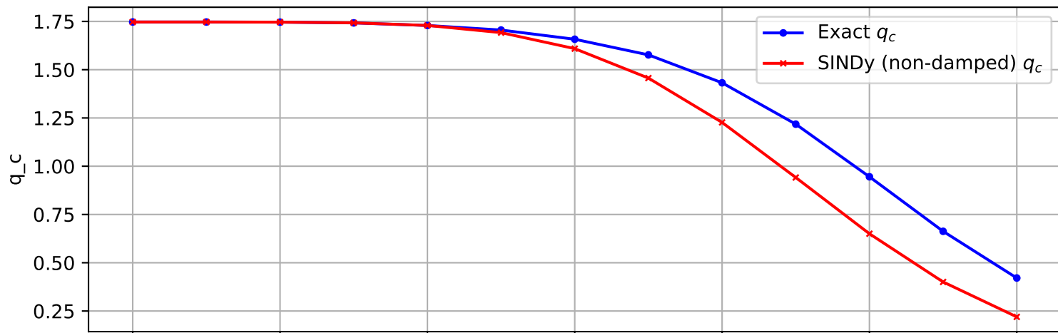
Trajectory 1625 (non-damped)
