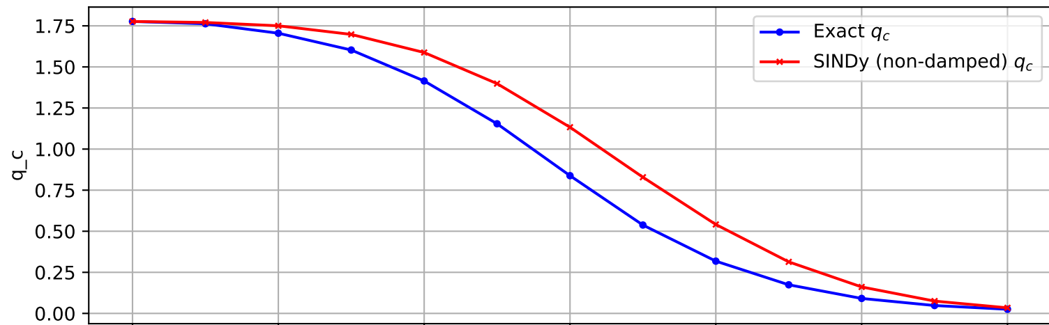
Trajectory 1631 (non-damped)
