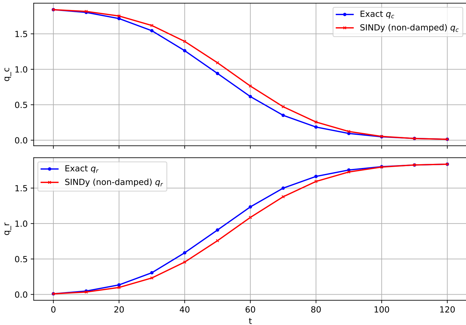
Trajectory 1638 (non-damped)
