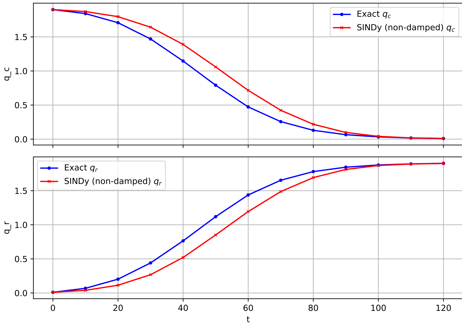
Trajectory 1643 (non-damped)
