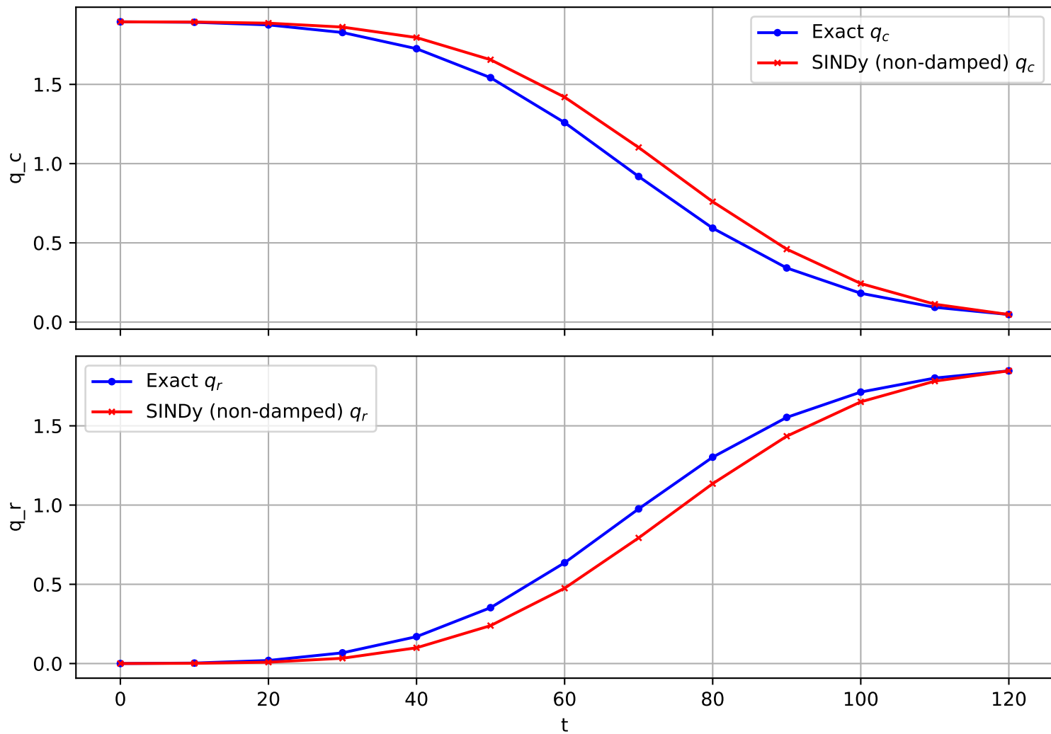
Trajectory 1645 (non-damped)
