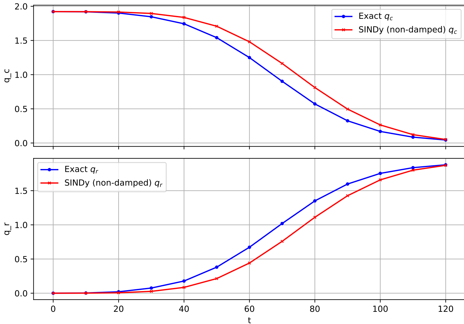
Trajectory 1647 (non-damped)
