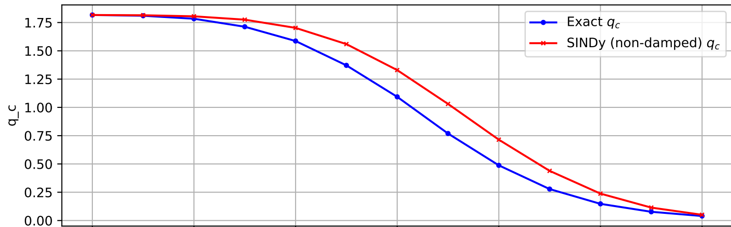
Trajectory 1654 (non-damped)
