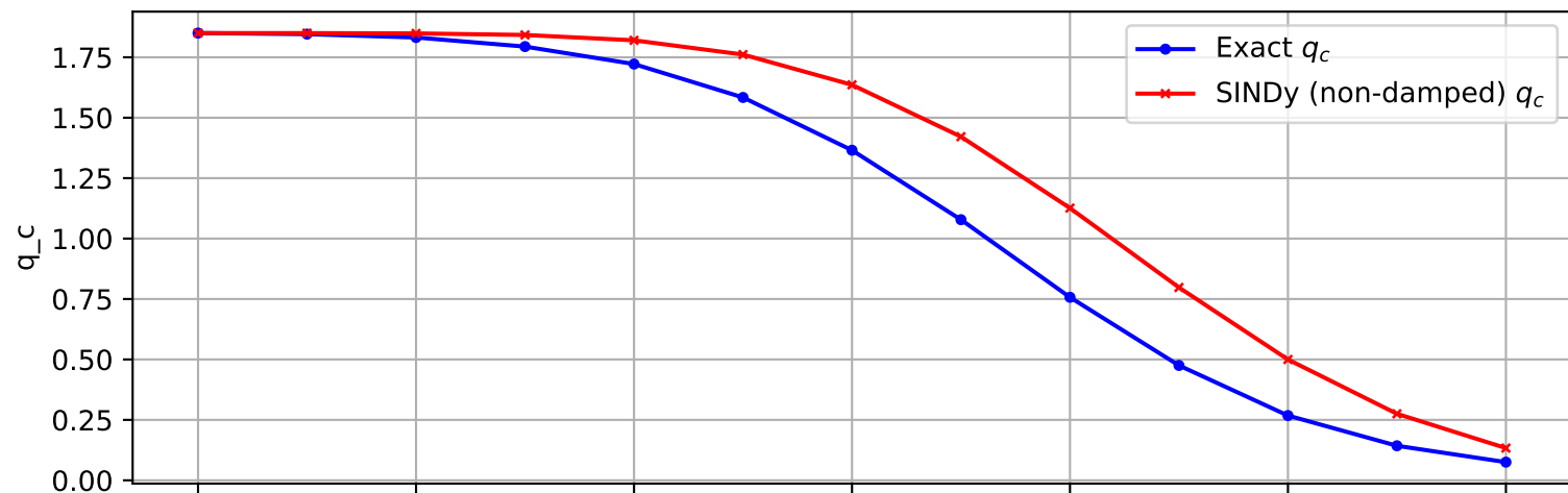
Trajectory 1656 (non-damped)
