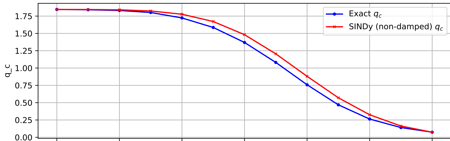
Trajectory 1661 (non-damped)
