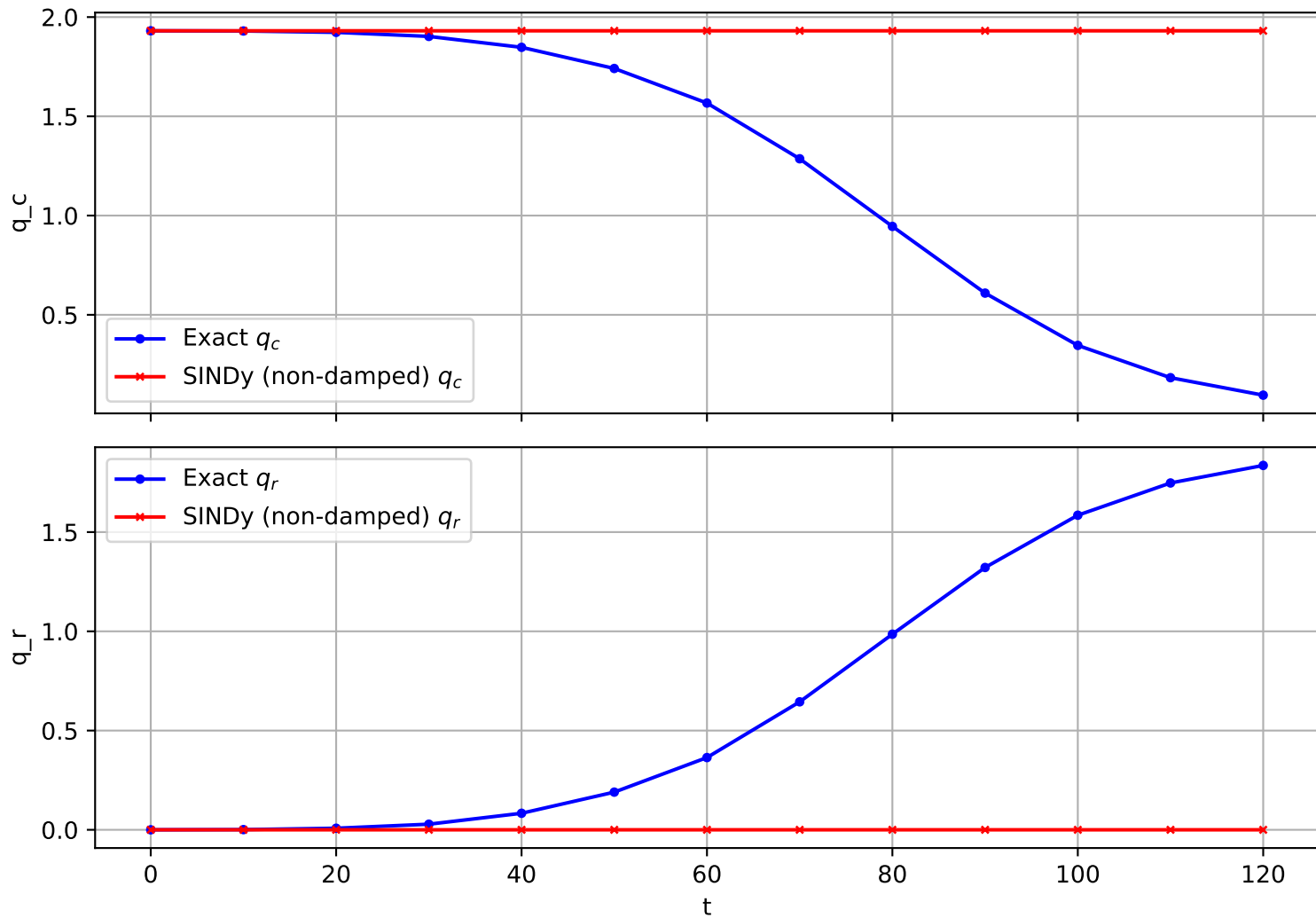
Trajectory 1668 (non-damped)
