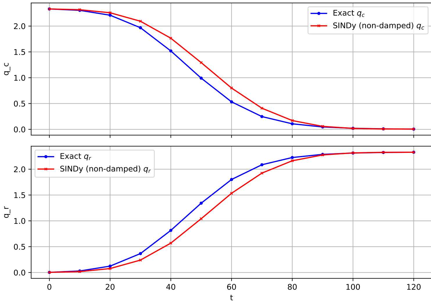
Trajectory 1684 (non-damped)
