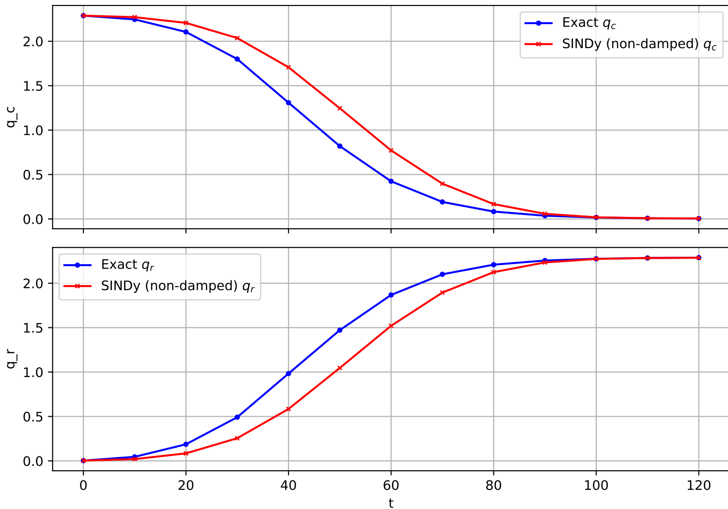
Trajectory 1686 (non-damped)
