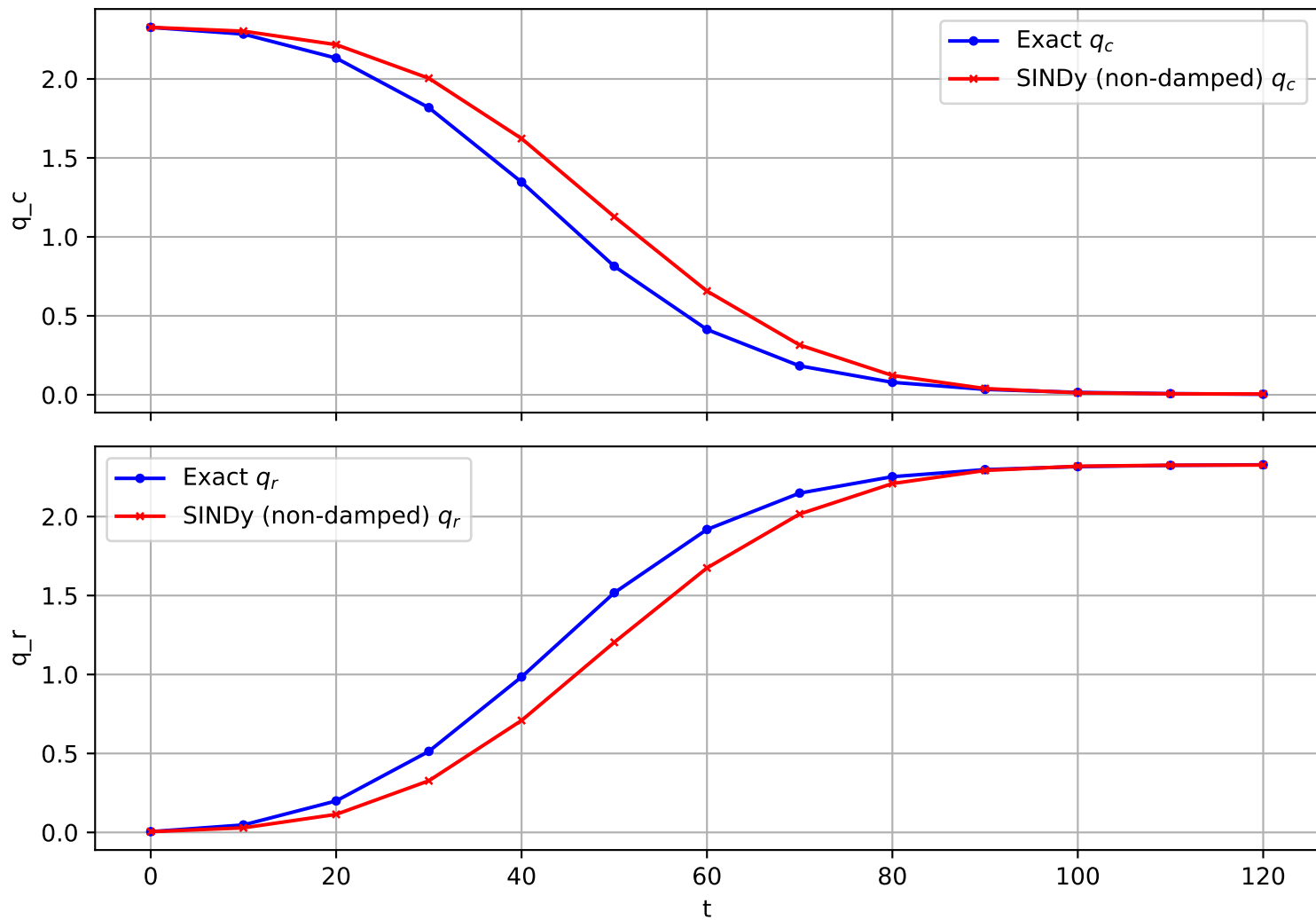
Trajectory 1689 (non-damped)
