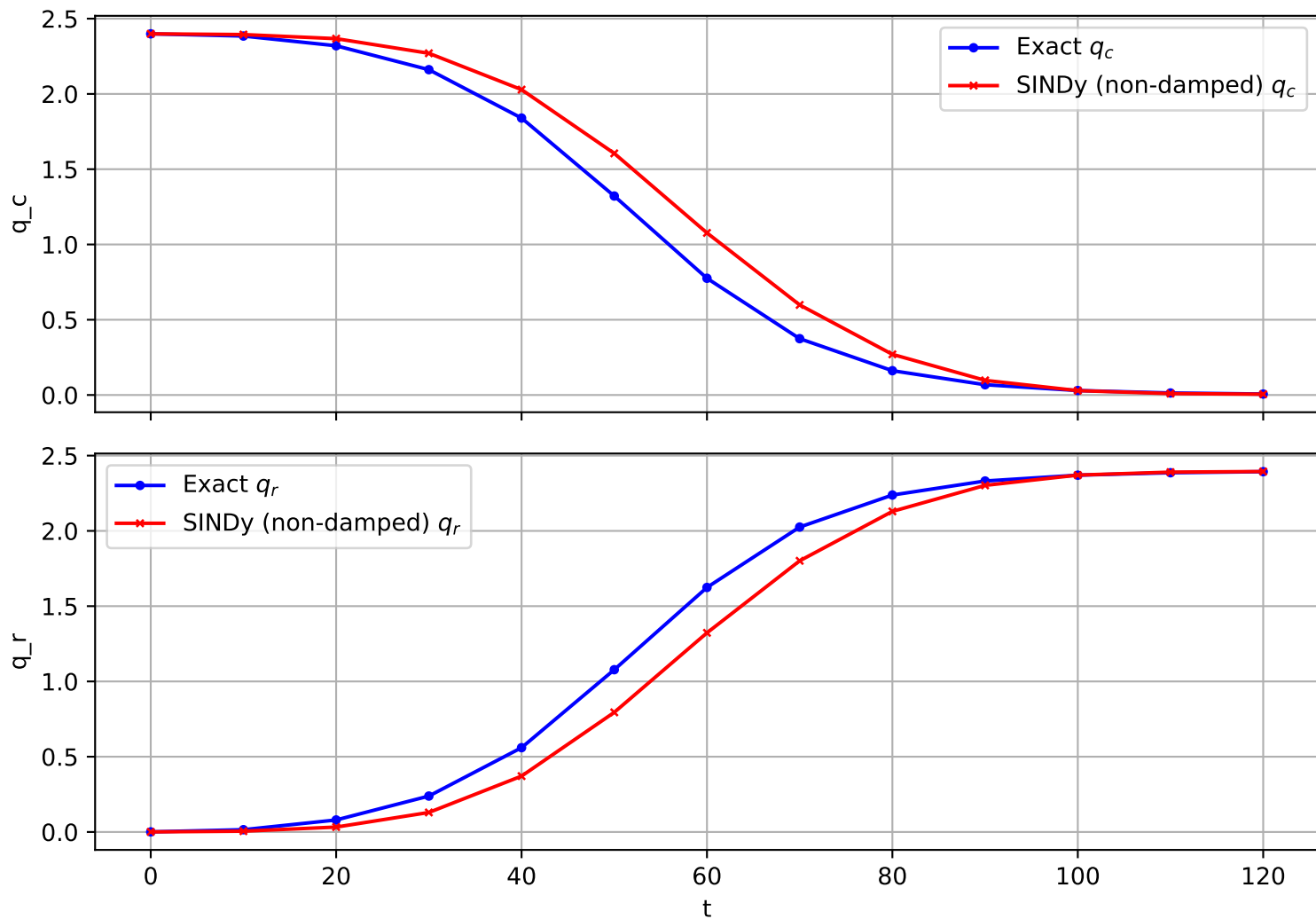
Trajectory 1694 (non-damped)
