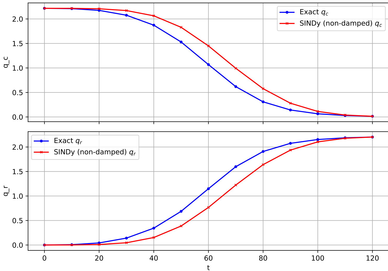
Trajectory 1704 (non-damped)
