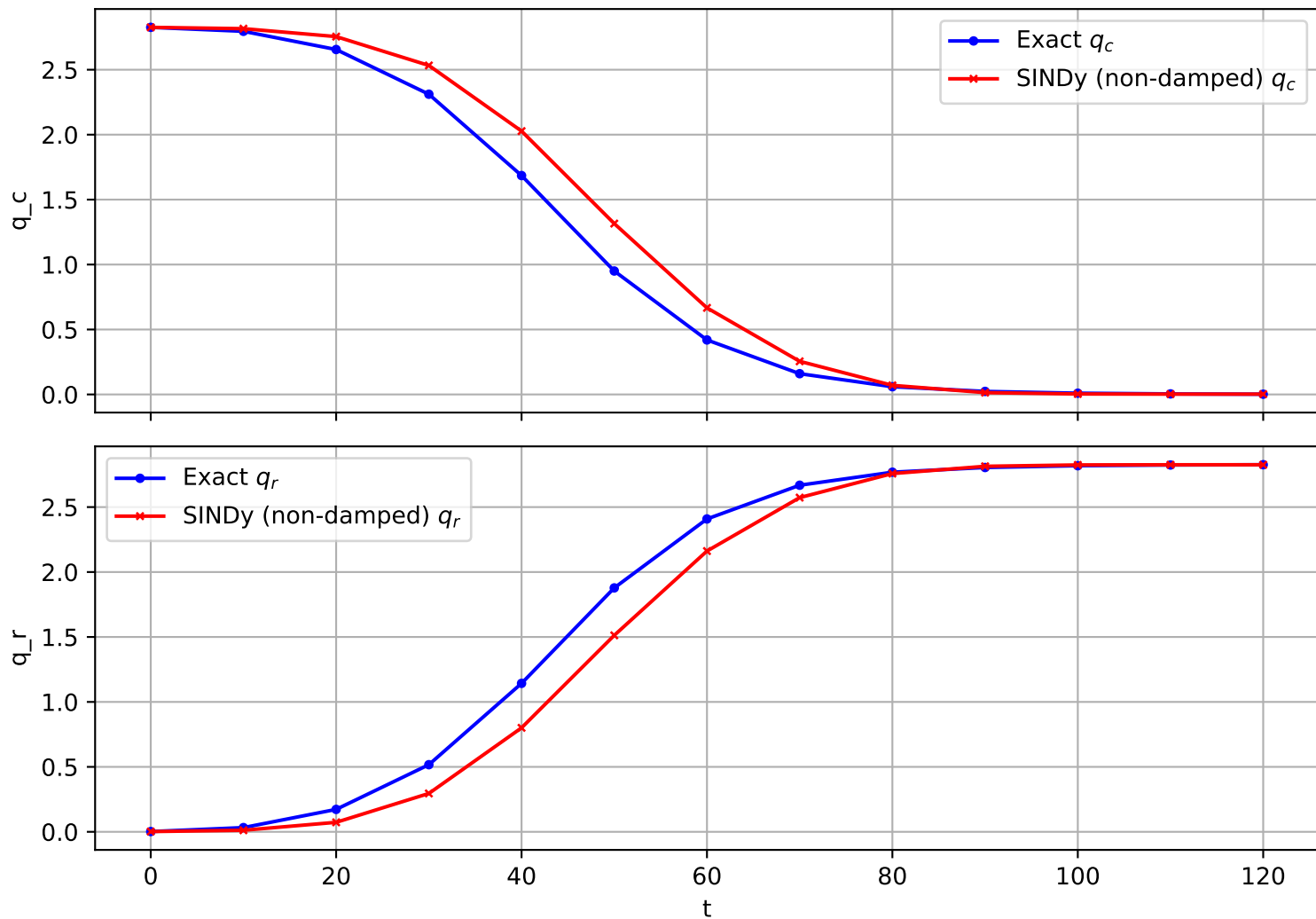
Trajectory 171 (non-damped)
