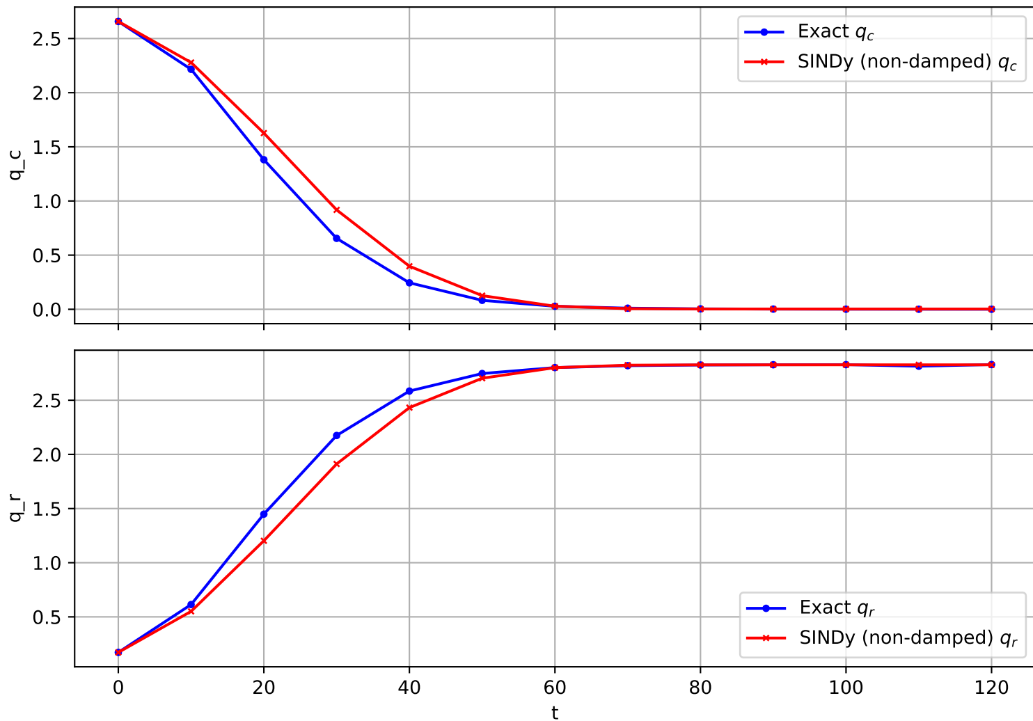
Trajectory 1711 (non-damped)
