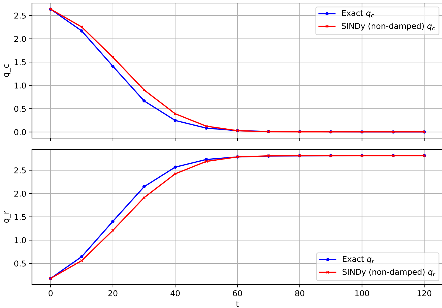
Trajectory 1713 (non-damped)
