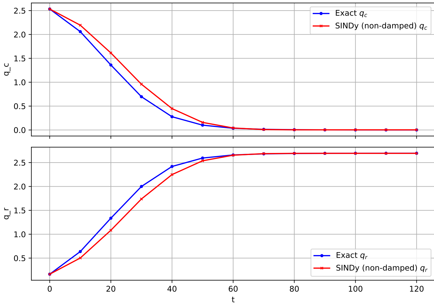
Trajectory 1714 (non-damped)
