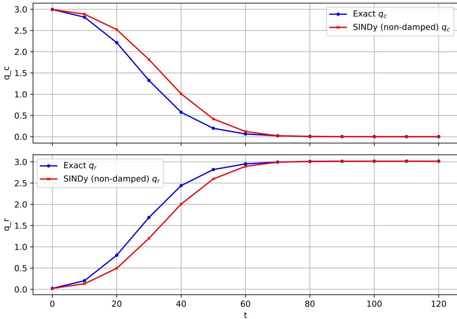
Trajectory 1717 (non-damped)
