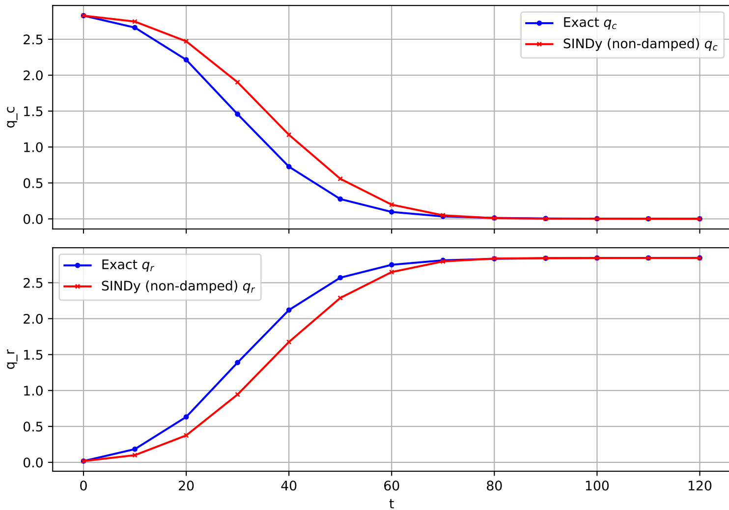
Trajectory 1718 (non-damped)
