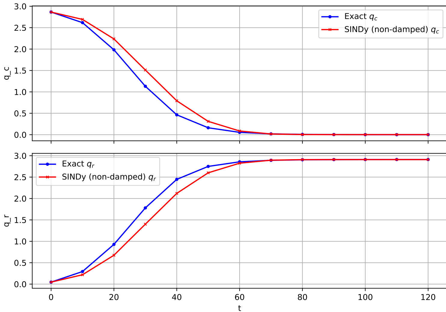
Trajectory 1721 (non-damped)
