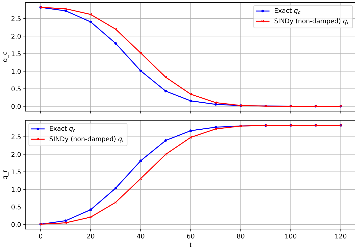
Trajectory 1725 (non-damped)
