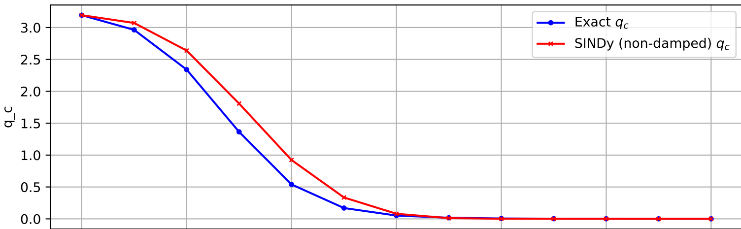
Trajectory 1763 (non-damped)
