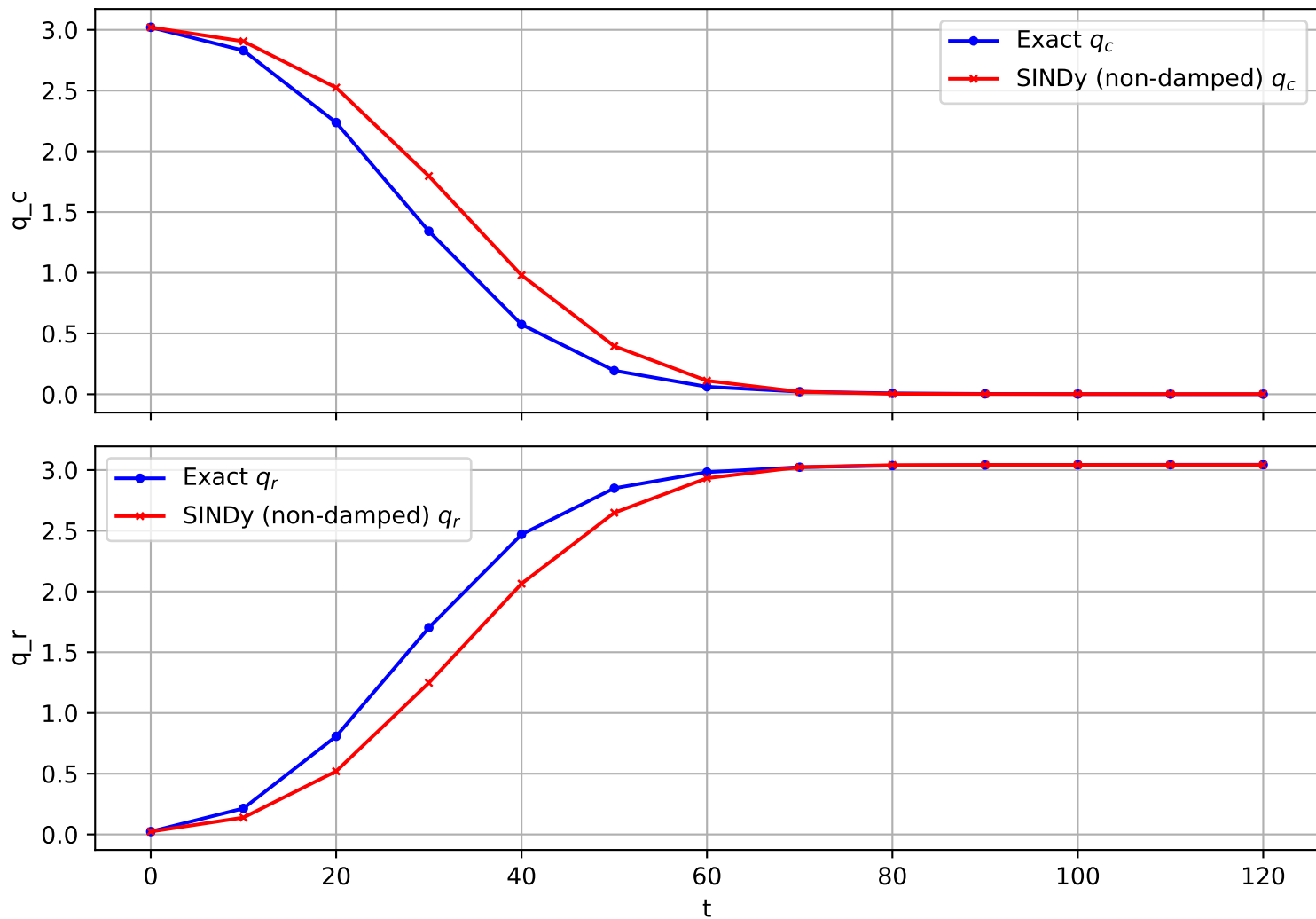
Trajectory 1764 (non-damped)
