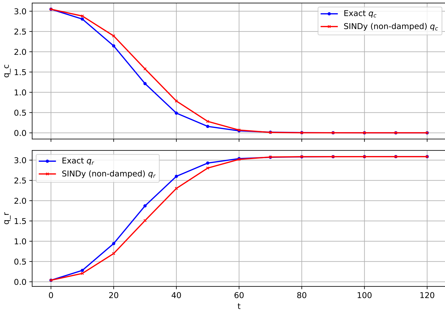
Trajectory 1765 (non-damped)
