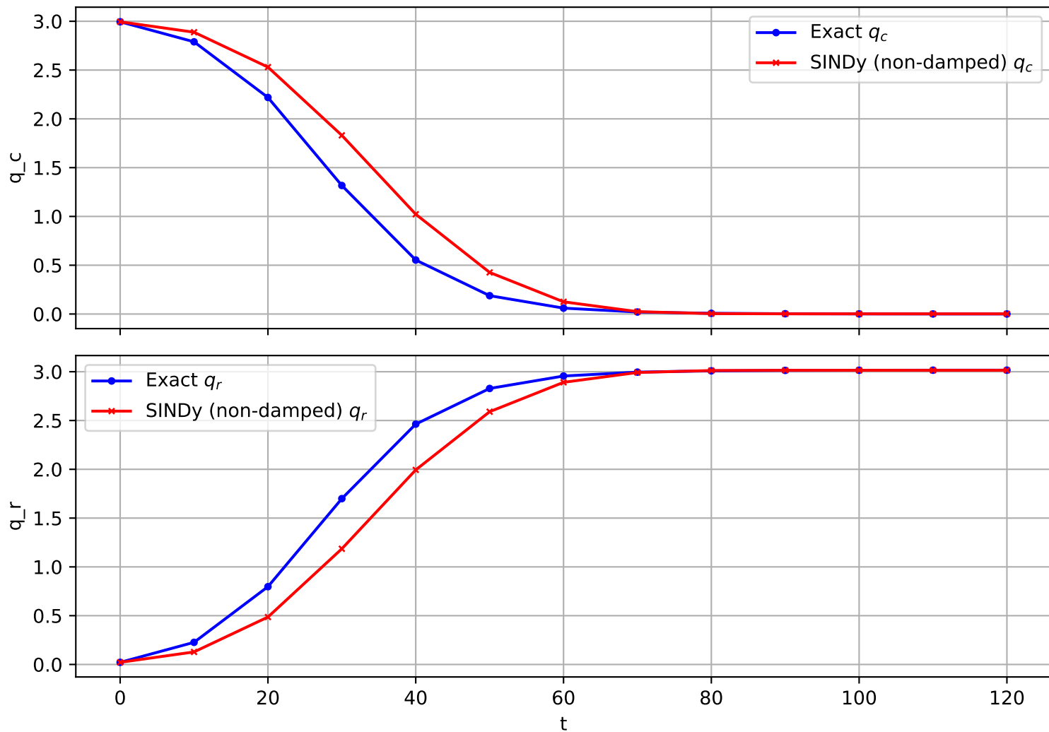
Trajectory 1766 (non-damped)
