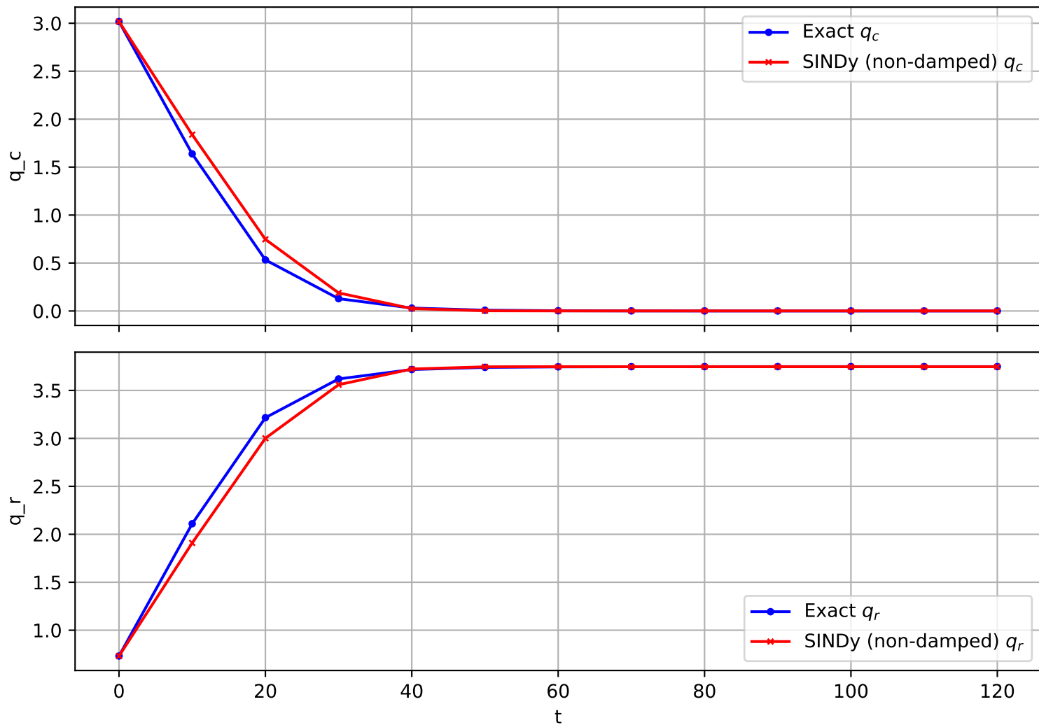
Trajectory 1782 (non-damped)
