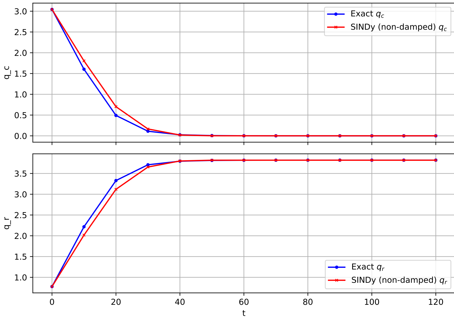
Trajectory 1785 (non-damped)
