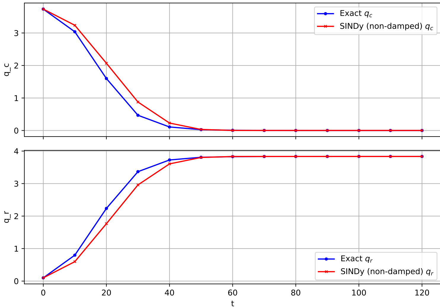
Trajectory 1800 (non-damped)
