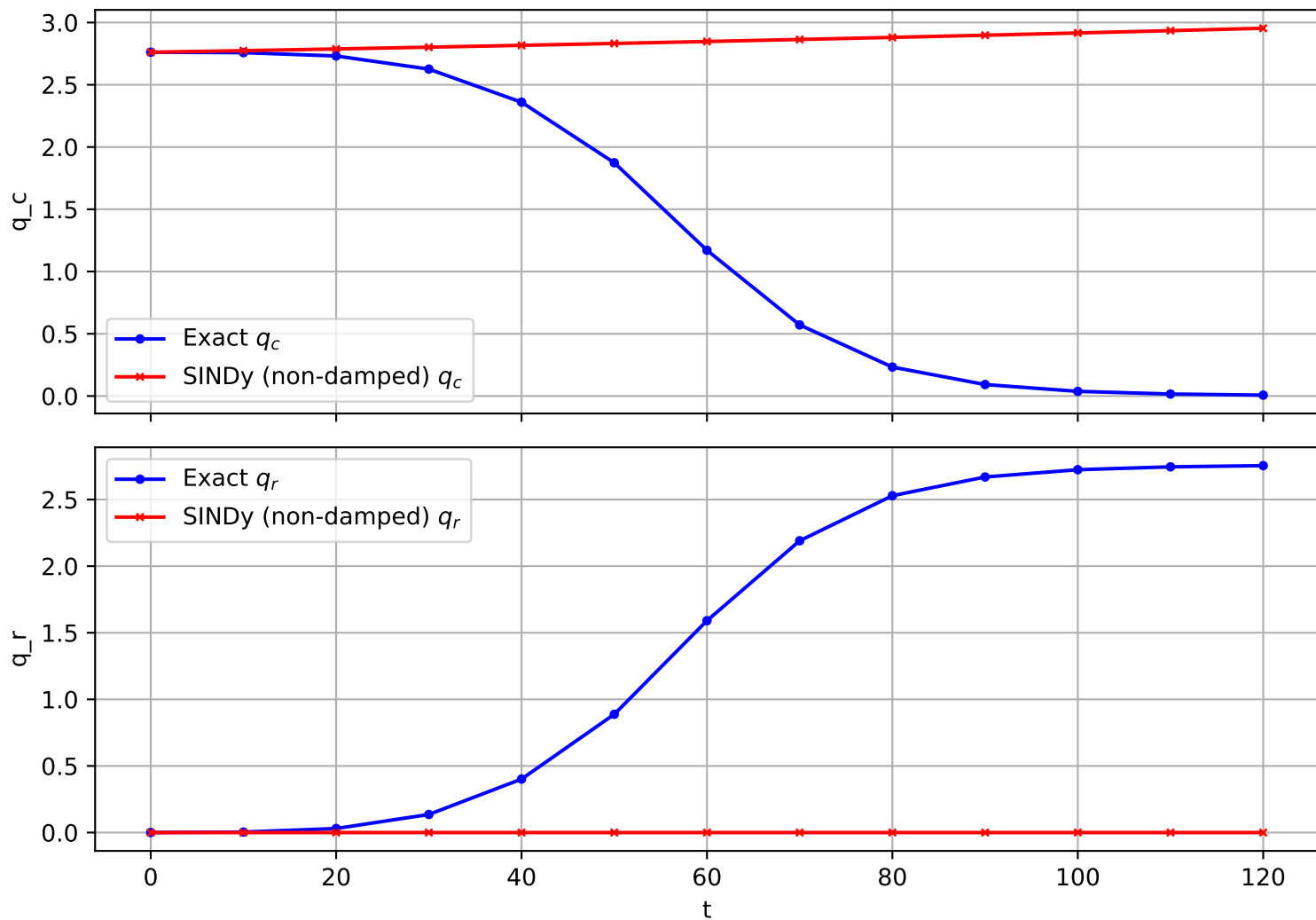
Trajectory 182 (non-damped)
