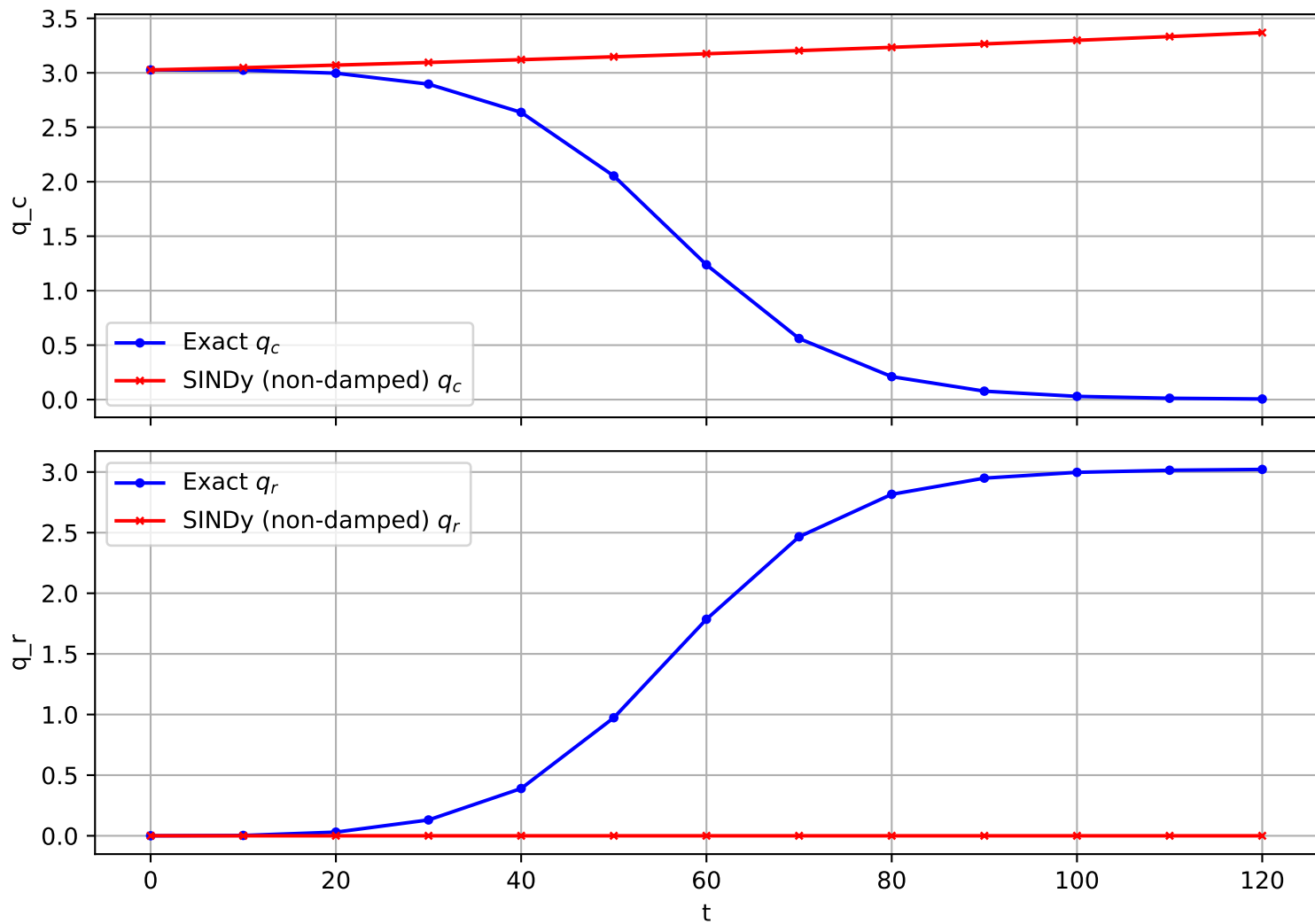
Trajectory 198 (non-damped)
