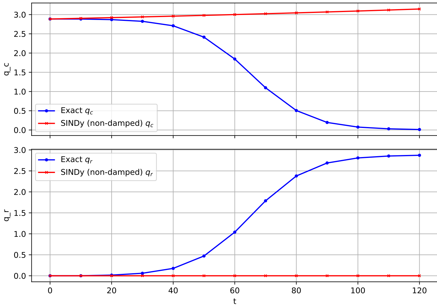
Trajectory 202 (non-damped)
