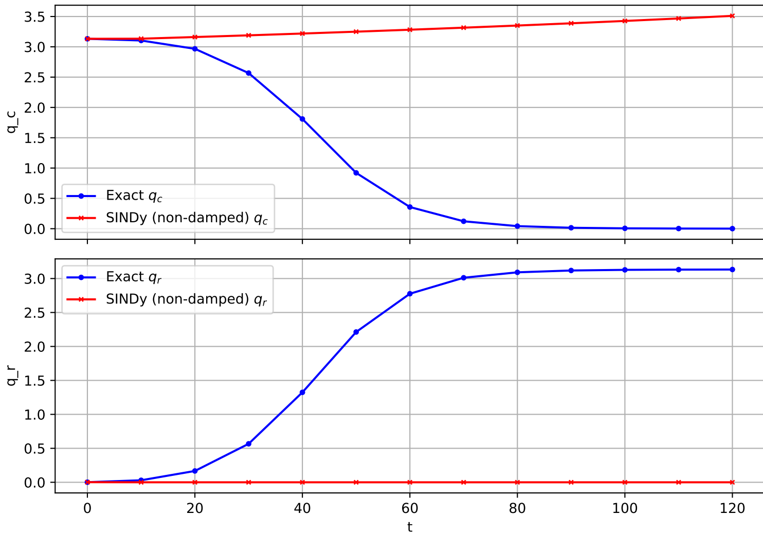
Trajectory 222 (non-damped)
