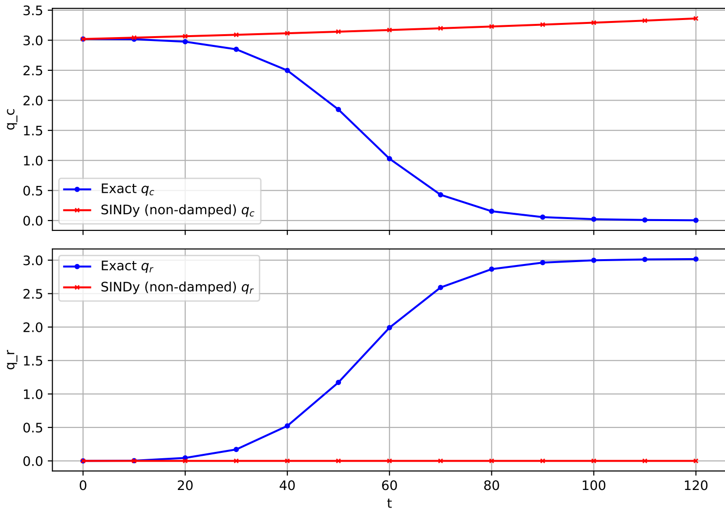
Trajectory 230 (non-damped)
