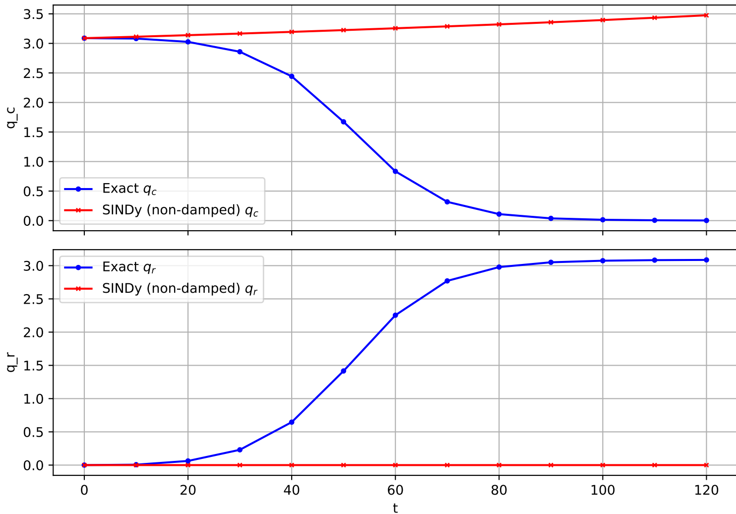
Trajectory 232 (non-damped)
