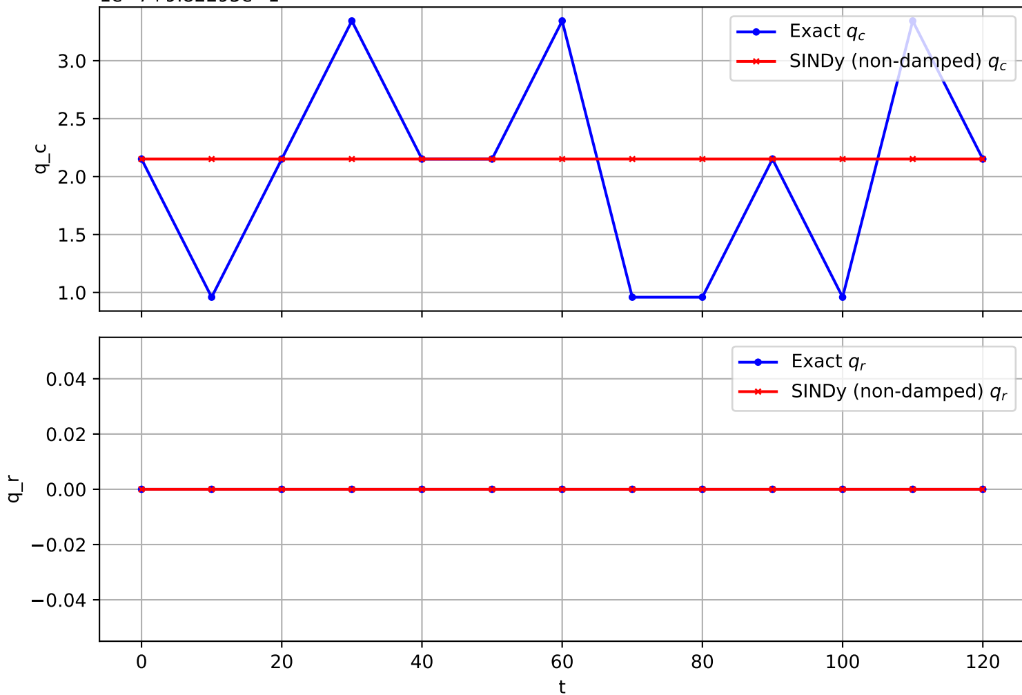
Trajectory 24 (non-damped)
