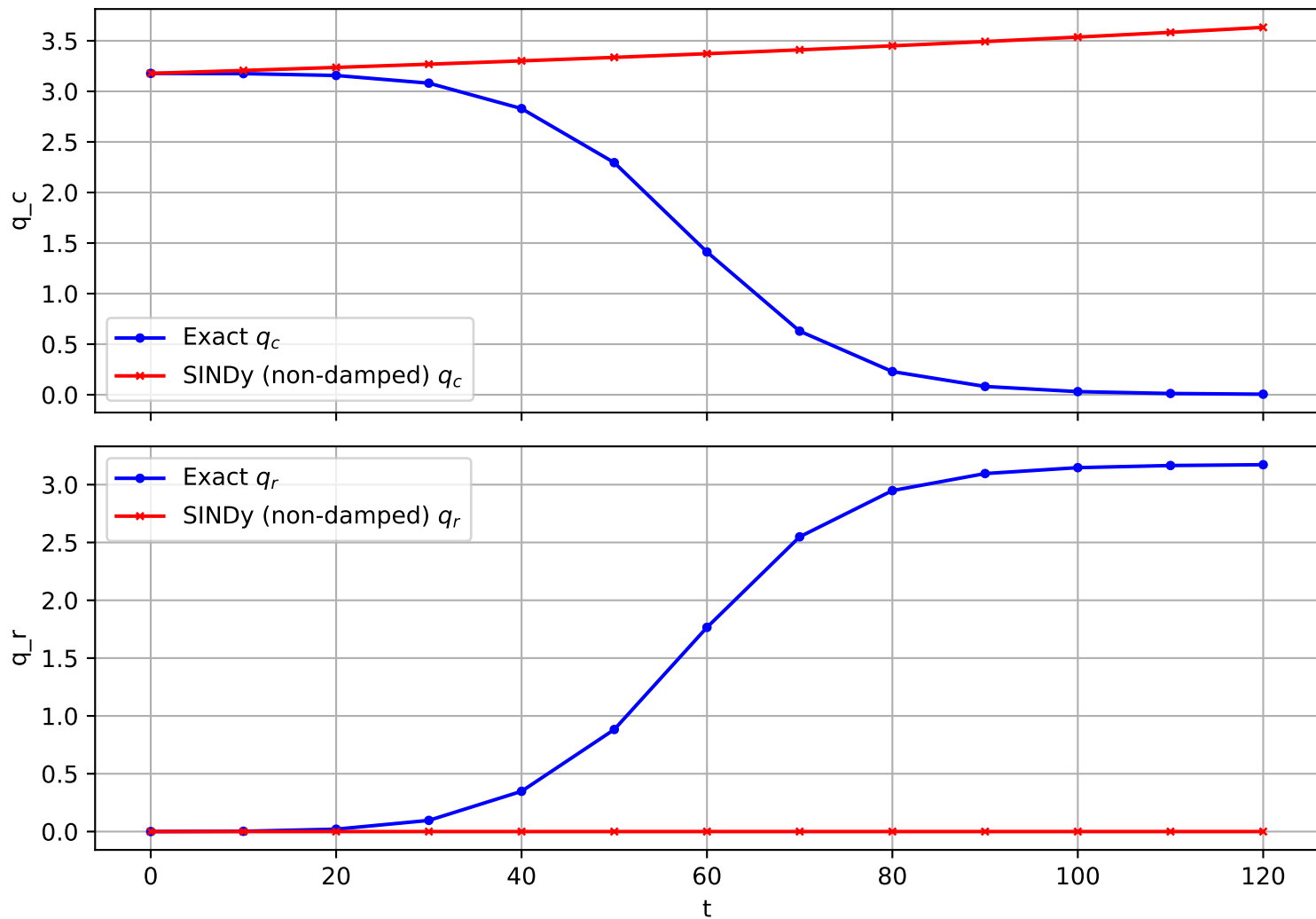
Trajectory 240 (non-damped)
