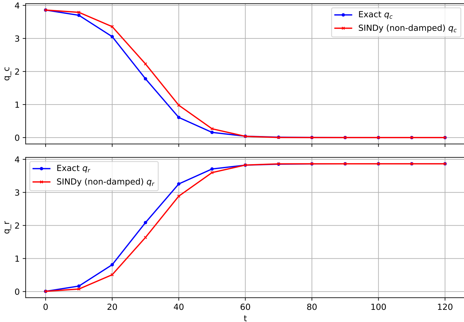
Trajectory 255 (non-damped)
