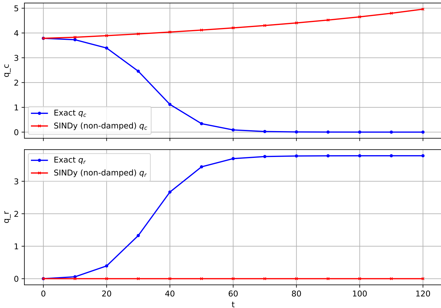
Trajectory 264 (non-damped)
