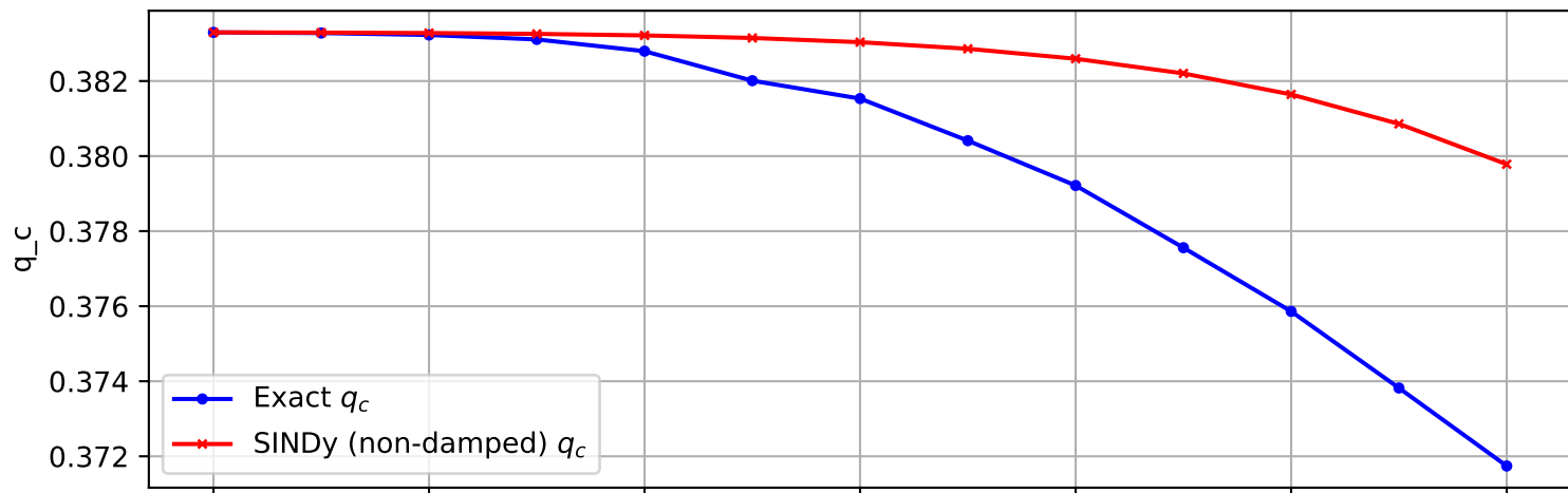
Trajectory 279 (non-damped)
