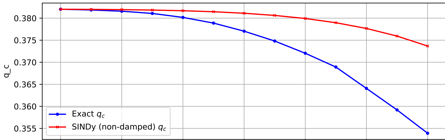
Trajectory 294 (non-damped)
